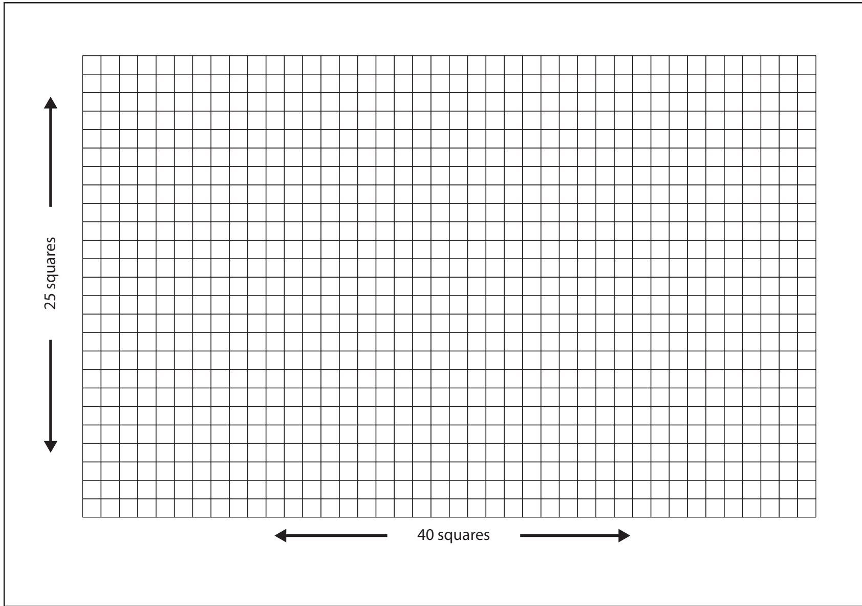
Fig. 2.20. Proportion of elements in 1,000 g seawater by mass Image by Byron Inouye
