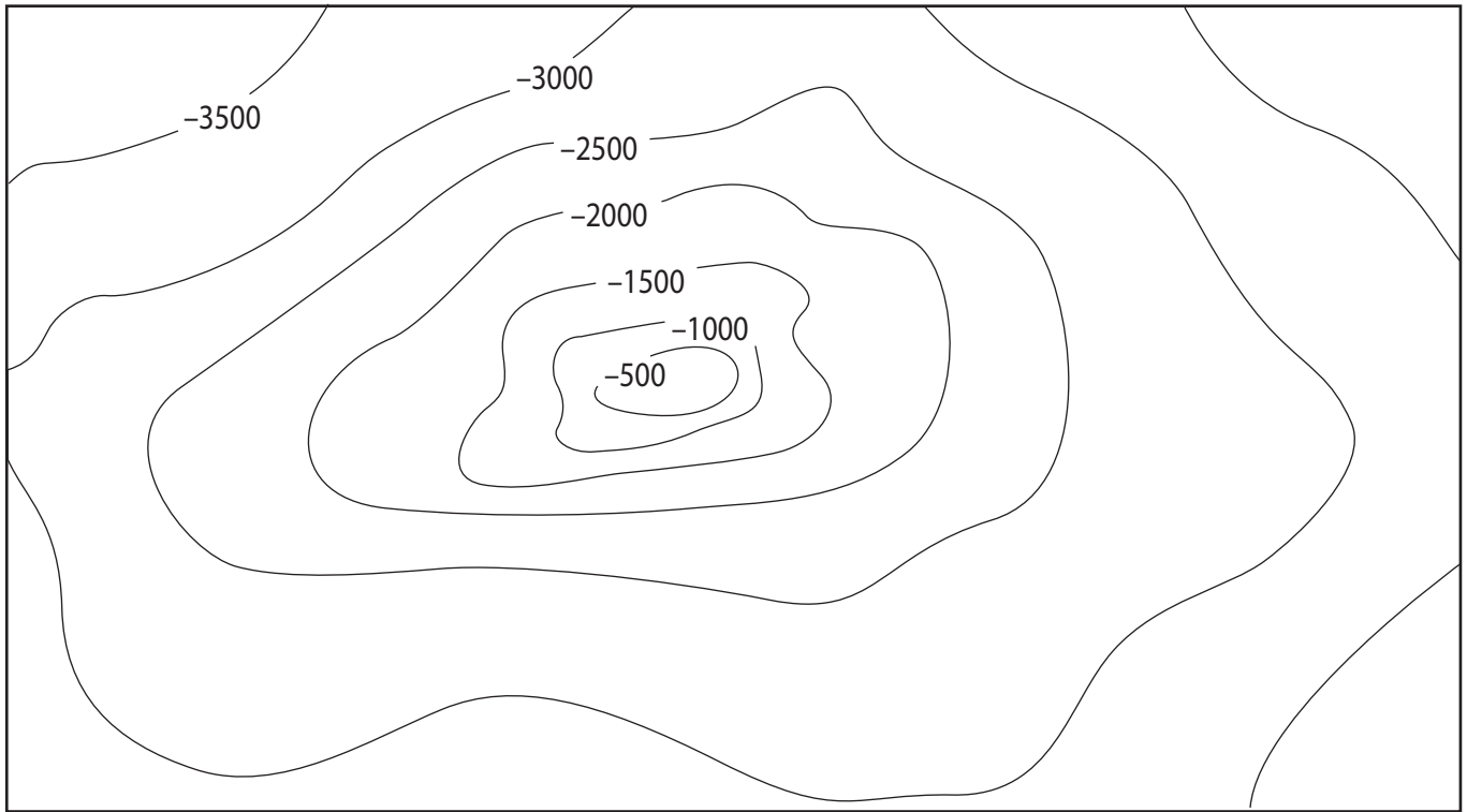
Fig. 7.37. Contour map H (elevation and depth in meters)
