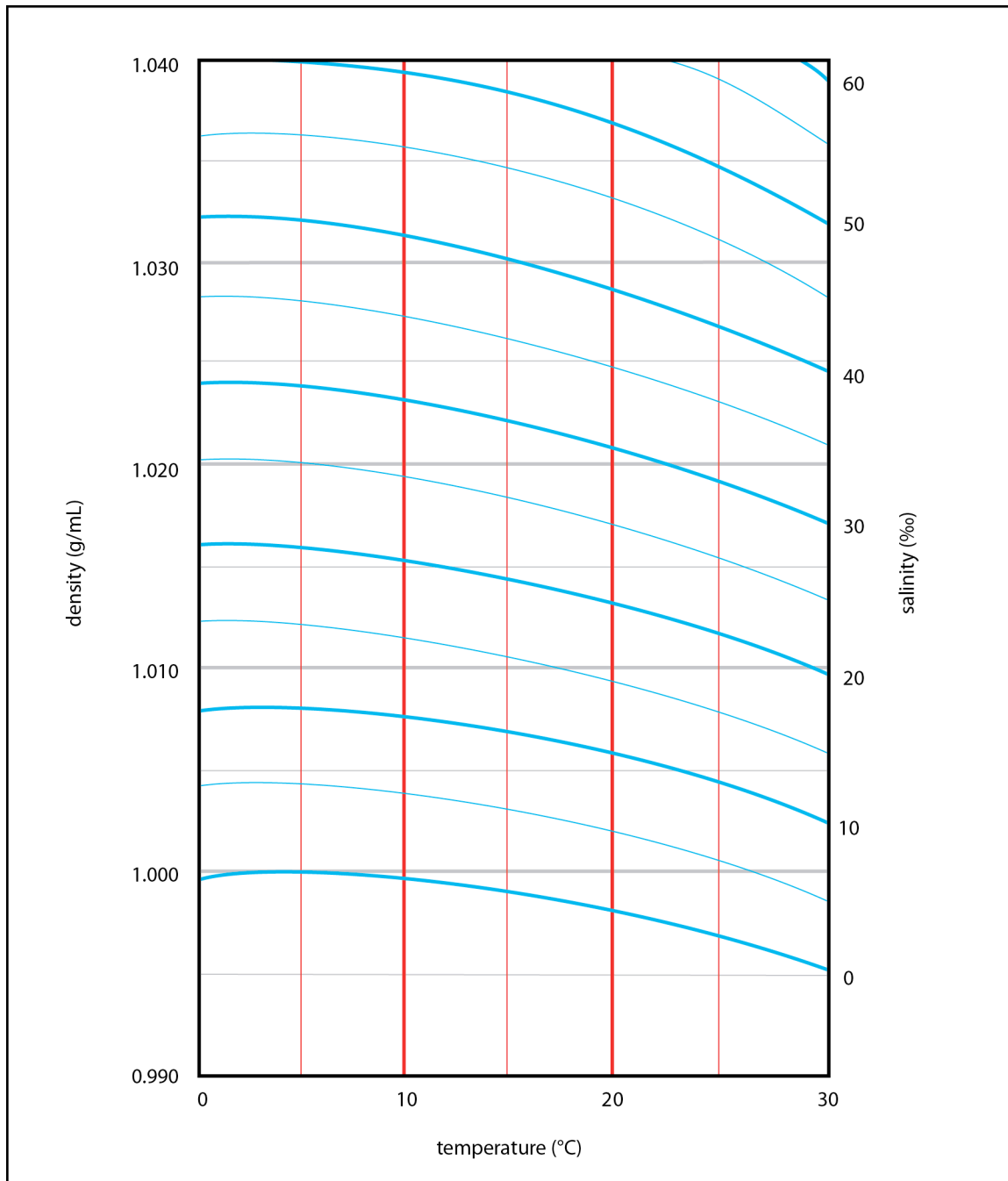
Fig. 2.13. Lines define relationships between temperature (red vertical lines), density (grey horizontal lines), and salinity (blue curved lines)
