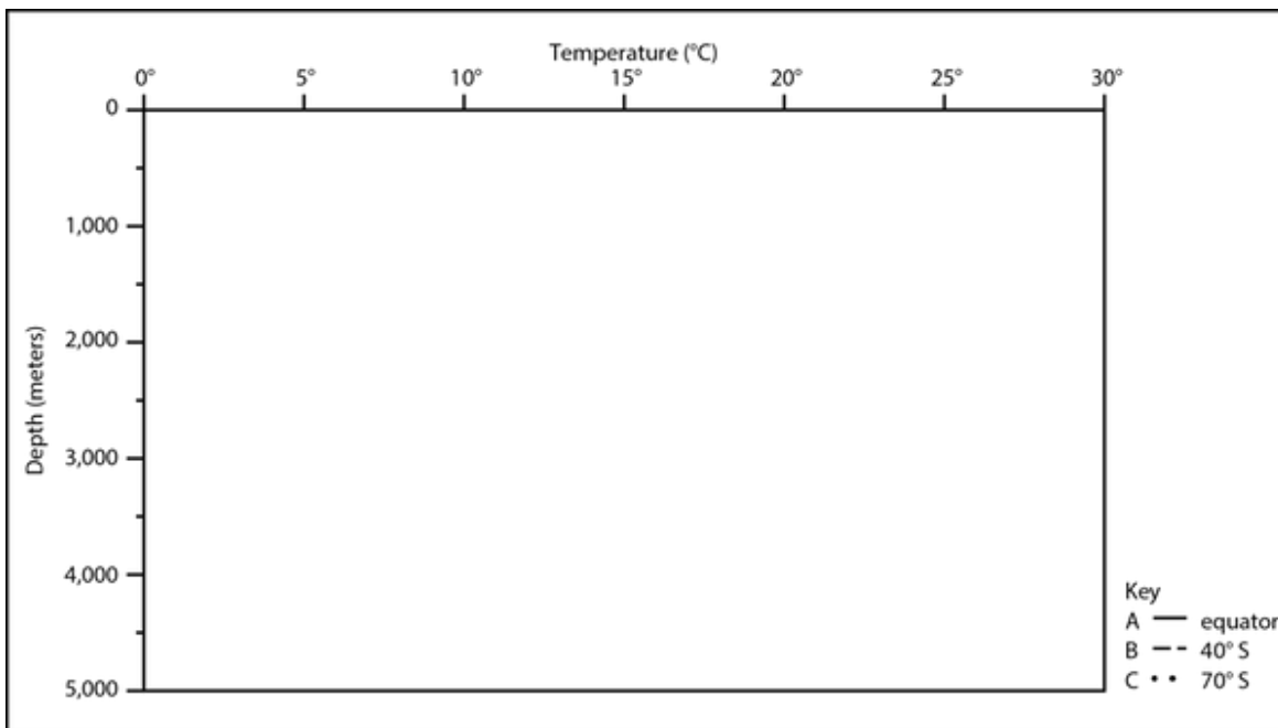
Fig. 2.11. Graph of the temperature of the Pacific ocean basin at (A) the equator, (B) 40° S latitude, and (C) 70° S latitude
