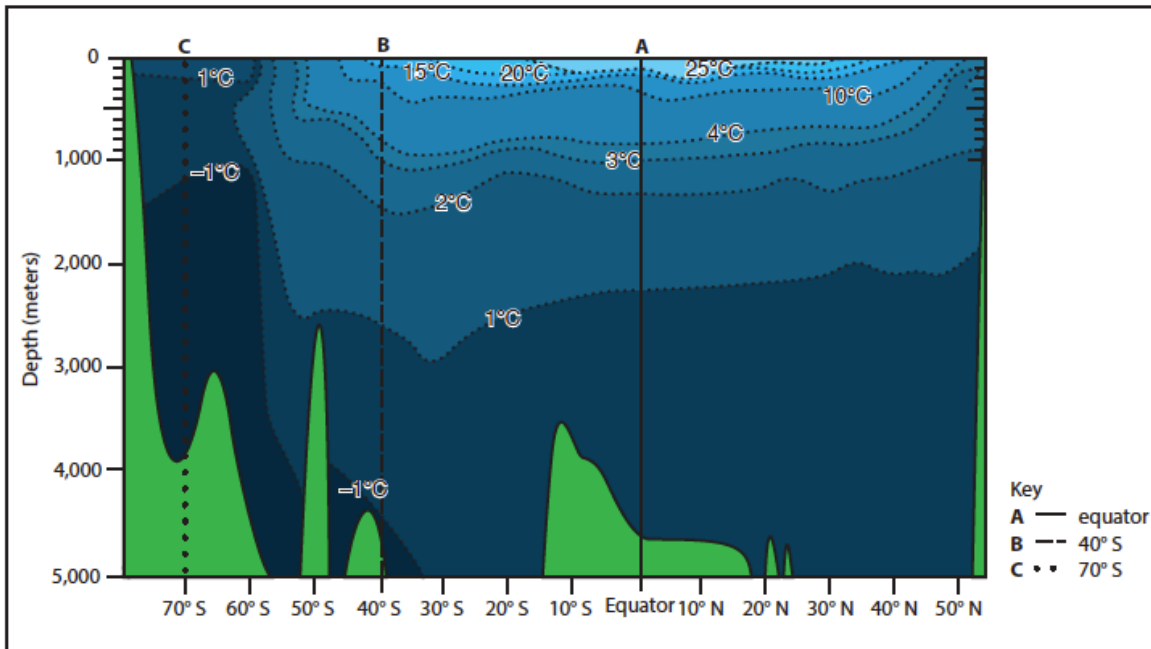
Fig. 2.10. Idealized vertical temperature profile of the Pacific ocean basin showing water in blue and seafloor features in green. The highest, or warmest, water temperatures are shown in light blue. The lowest, or coldest, water temperatures are shown in dark blue.
